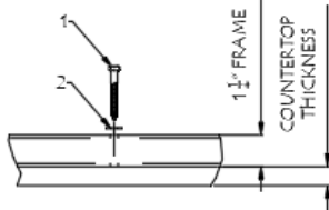
SCREW
