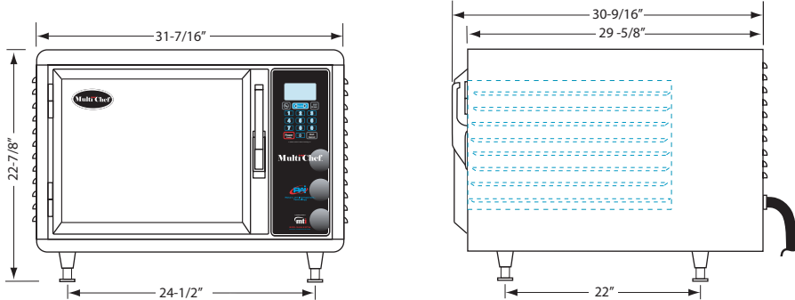
Multi-Chef Oven
