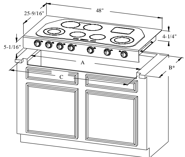
Fig. B – CTE48P Installed with End Caps
