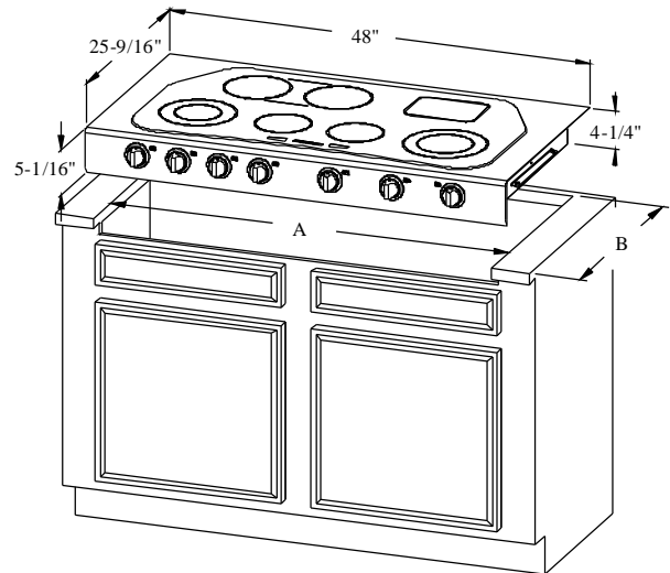
Fig. A – CTE48P Installed without End Caps
