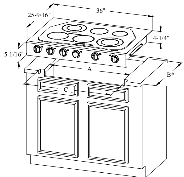
Fig B - CTE36P Installed with End Caps
