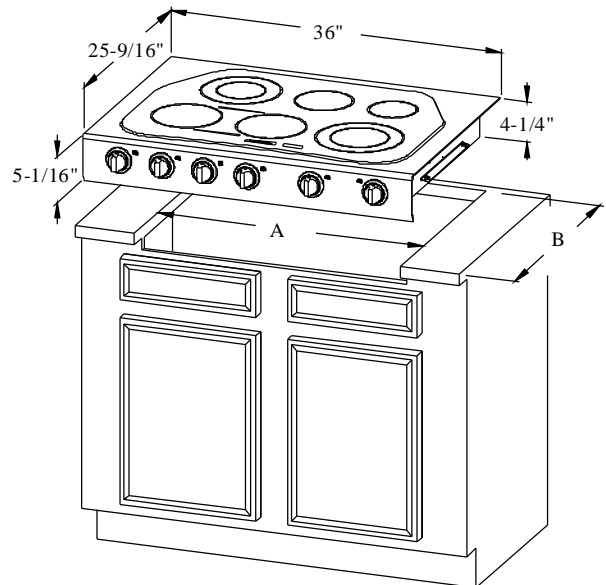
Fig A - CTE36P Installed without End Caps
