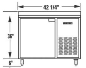
DLFB42-SS-BS FRONT VIEW
