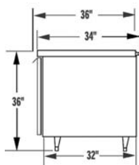
DLFB-SS SIDE VIEW
