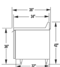
DLFB-SS-BS SIDE VIEW
