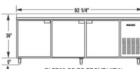
DLFB92-SS-BS FRONT VIEW
