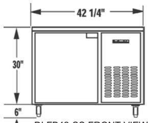
DLFB42-SS FRONT VIEW
