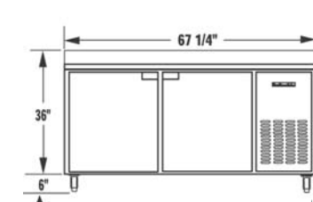
DLFB67-SS-BS FRONT VIEW
